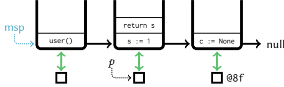
Fig. 4. Before capturing the continuation.
