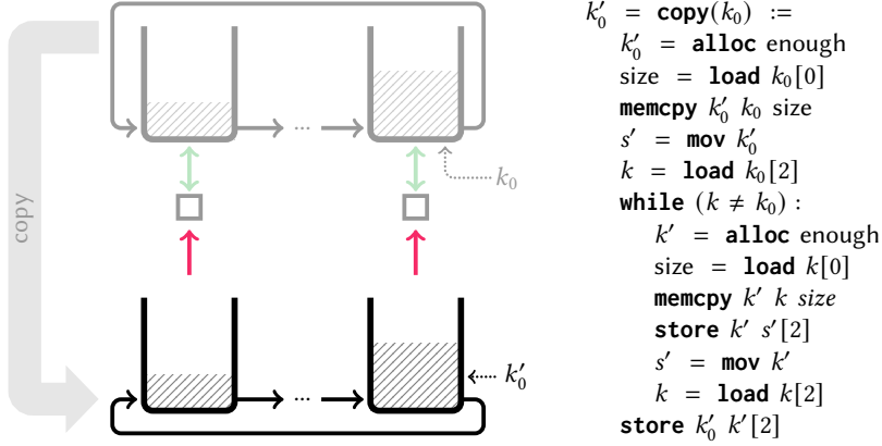
Fig. 13. Copying a continuation k (greyed out, since it remains unchanged) results in a deep copy of each stack with invalid prompt pointers. That is, the prompt does not point back to the copy of the stack.
