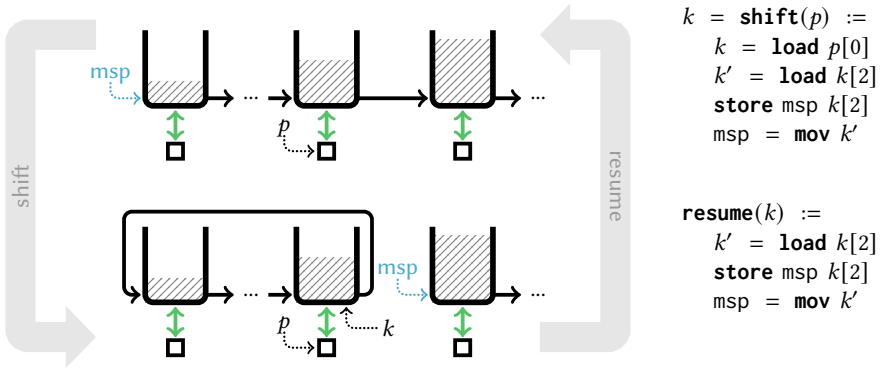
Fig. 12. Shift and resume only amounts to switching two pointers.
